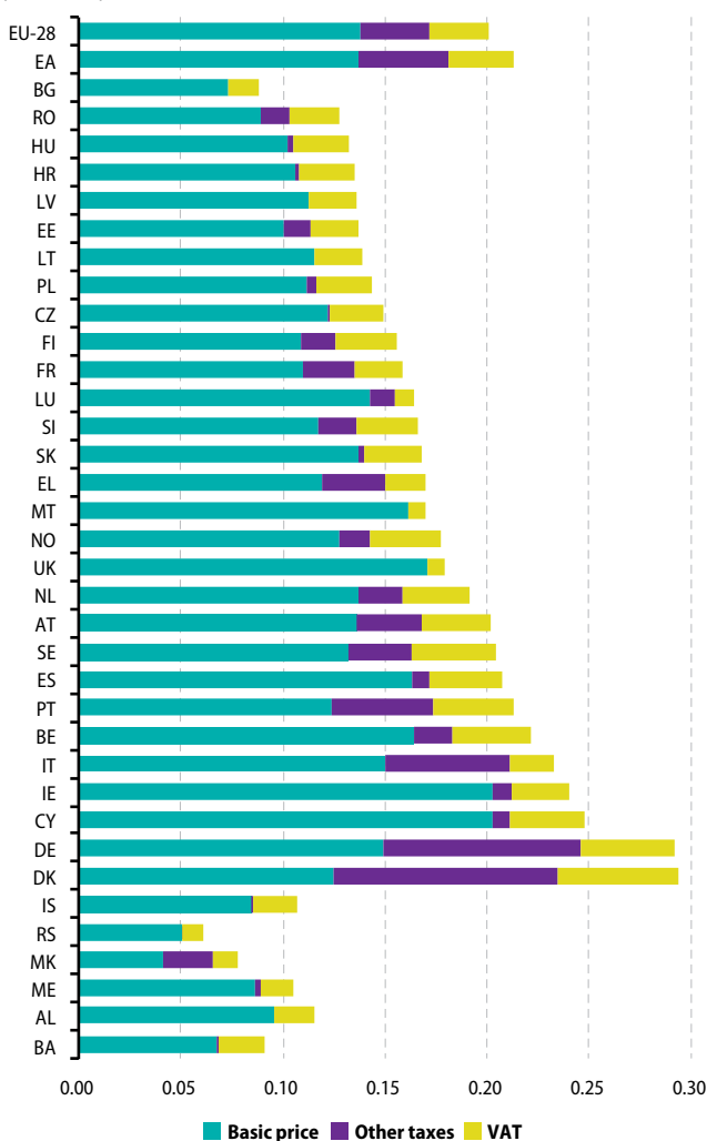
Figure 2.1.1: Electricity prices for household consumers, 2 nd semester 2013 (EUR/kWh)
